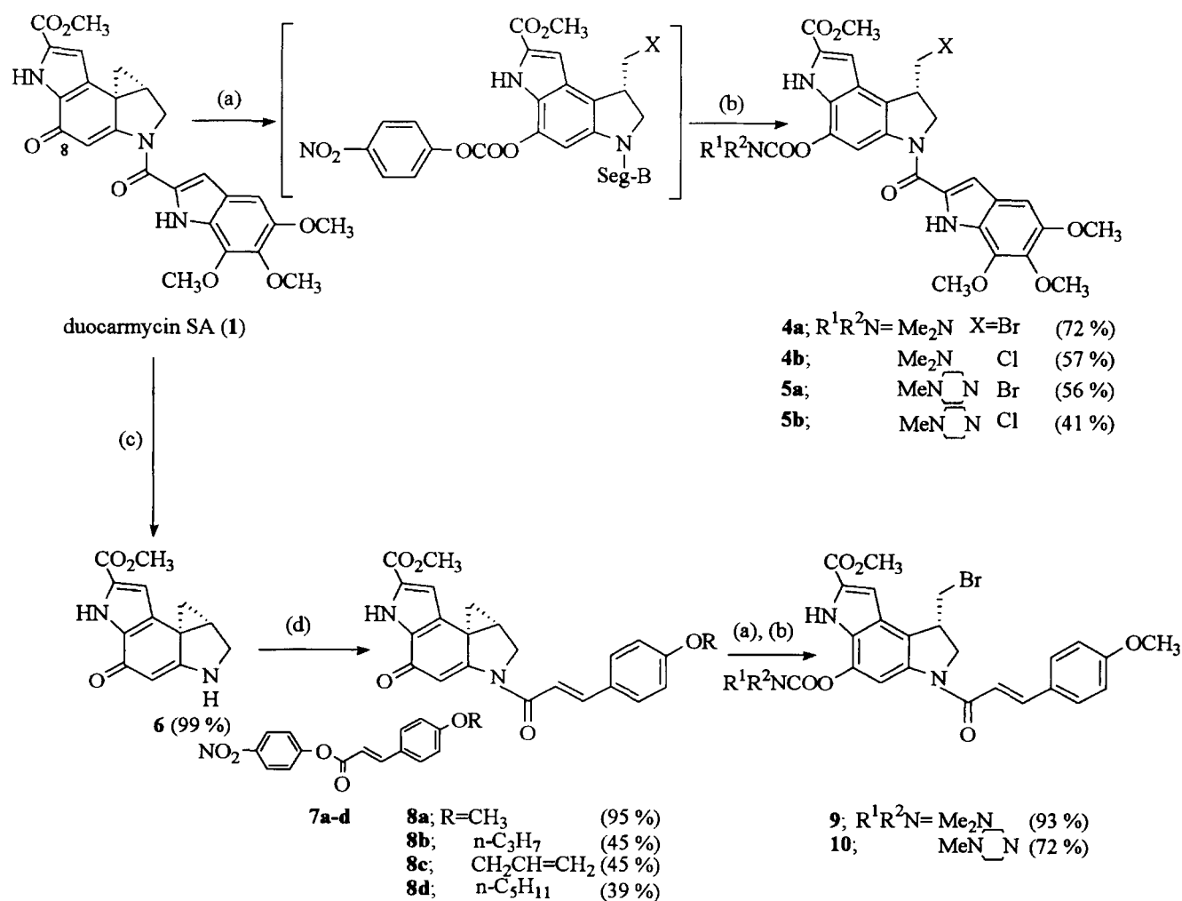
Figure 1. Structures of duocarmycins, CC-1065 and duocarmycin derivatives.
